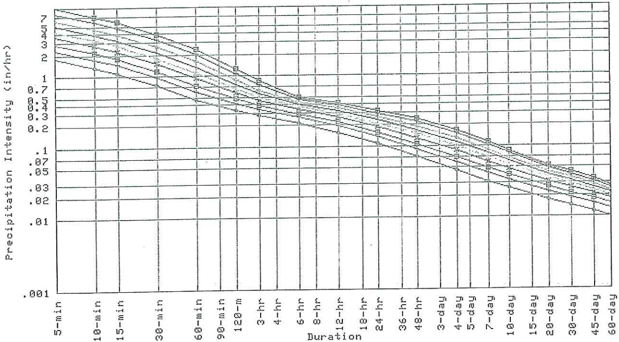
Partial duration based Point IDF Curves 38.95 N 119.94 W 6541 ft
